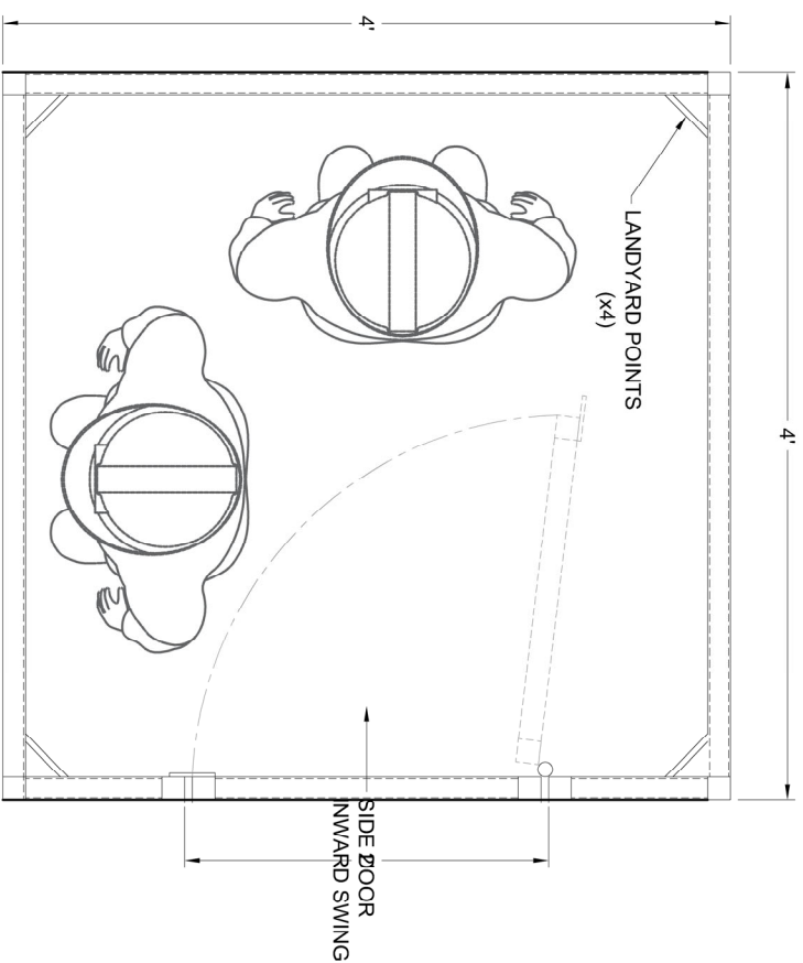
PLAN VIEW
